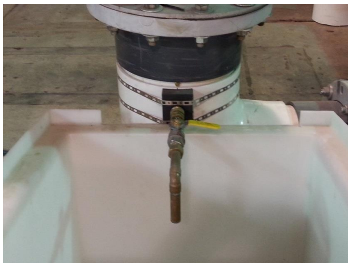
Figure 11 Photograph Showing the Background Isokinetic Sampler
