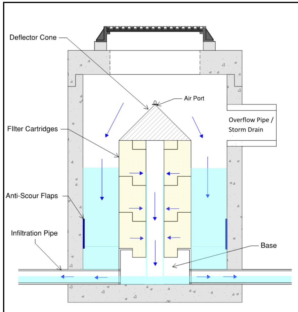
Figure 1 Hydroworks HydroFilter Operation – Low Flow
