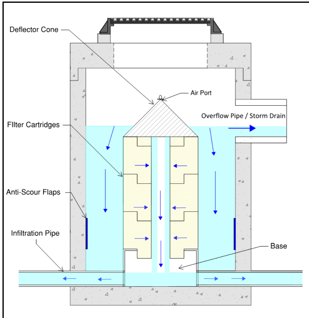
Figure 2 Hydroworks HydroFilter Operation – Bypass
