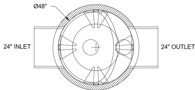
Figure 1B Plan View of the Barracuda MAX S4 Model Test Unit
